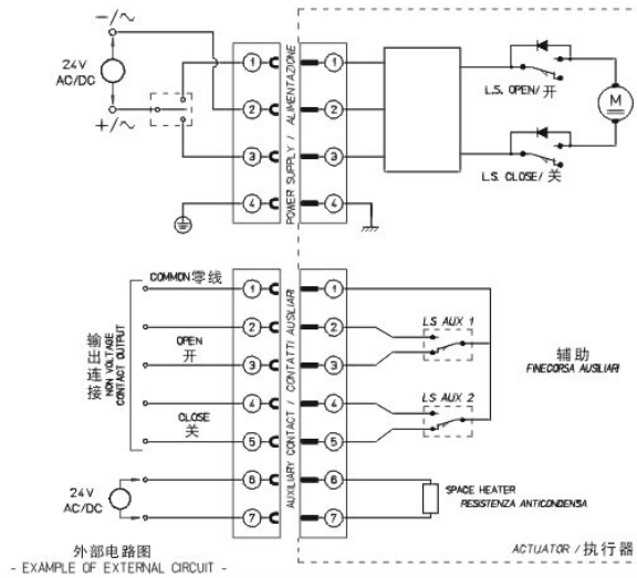
电气线路24 Vac/dc - 24 Vdc ELECTRIC WIRING FOR 24 Vac/dc - 24 Vdc SUPPLY
