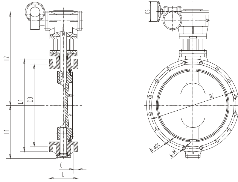
BUTTERFLY VALVE WITH GEAR BOX 手动蜗轮蝶阀
