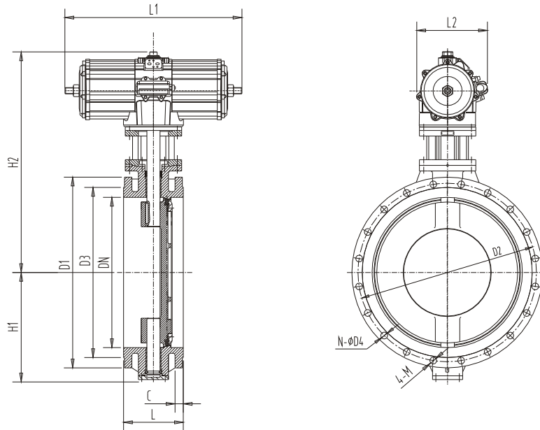
ACTUATED VALVE WITH DOUBLE ACTING PNEUMATIC ACTUATOR 双动气动蝶阀
